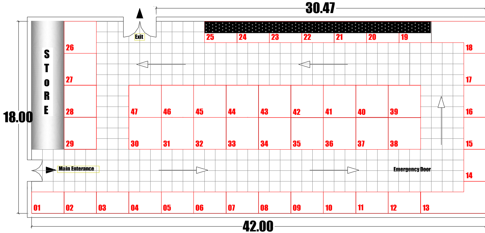
PAVILION-2 Partition Layout scale 1:200
