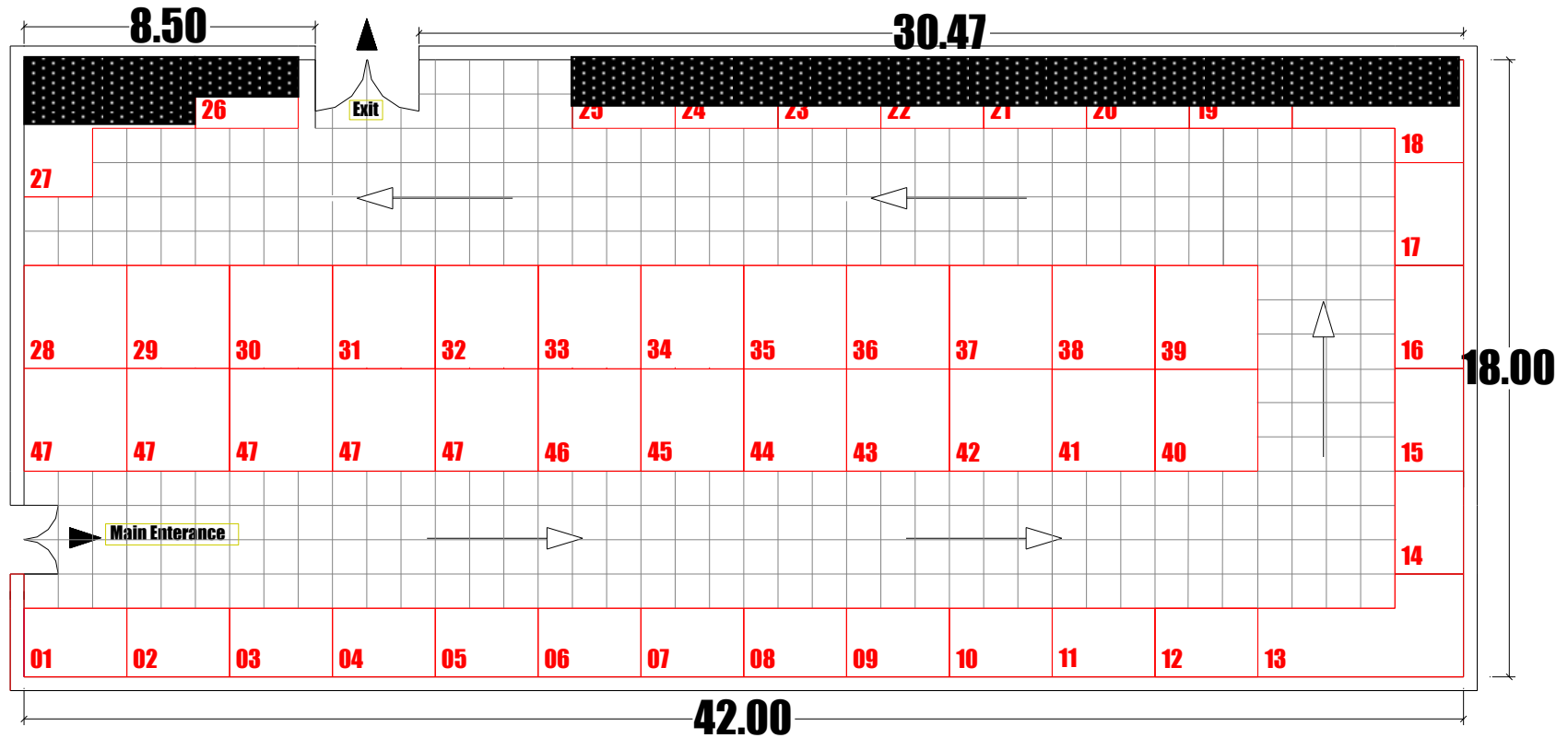
PAVILION-3 Partition Layout scale 1:200
